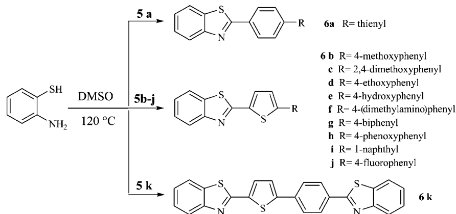
Scheme 2. Synthesis of benzothiazoles 6a–k .
