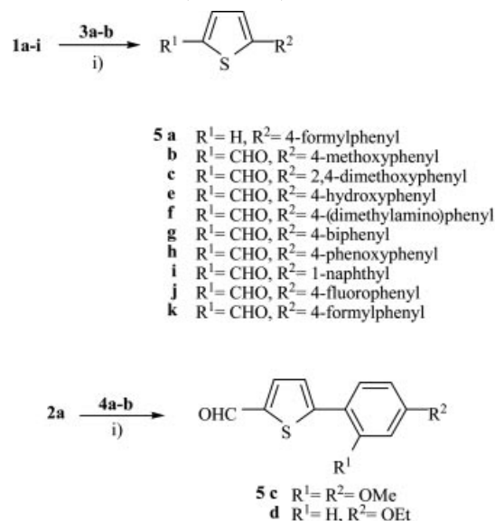
Scheme 1. Synthesis of formyl derivatives 5a–k by Suzuki coupling. Reagents and conditions: (i) DME, Pd(PPh 3 ) 4 (6 mol-%), Na 2 CO 3 (2 M), 80 °C, Ar.
