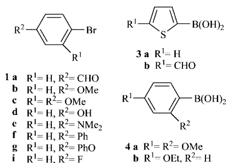
Figure 1. Structures of compounds 1 and 3–4 .
