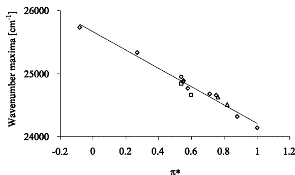
Figure 3. Correlation between absorption wavenumbers \tilde{\nu}_{\max} and the \pi^* scale according to Kamlet and Taft for compound 6f . Solvents: apolar and polar aprotic ( \diamond ), protic ( \square ), chlorinated ( \Delta ) and aromatic ( \circ ).
